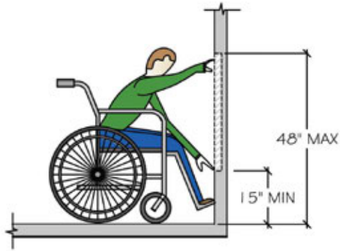
UNOBSTRUCTED FORWARD REACH
