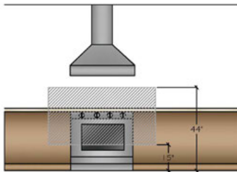
VENTILATION CONTROLS WITHIN 15"-44" REACH CONTROL
